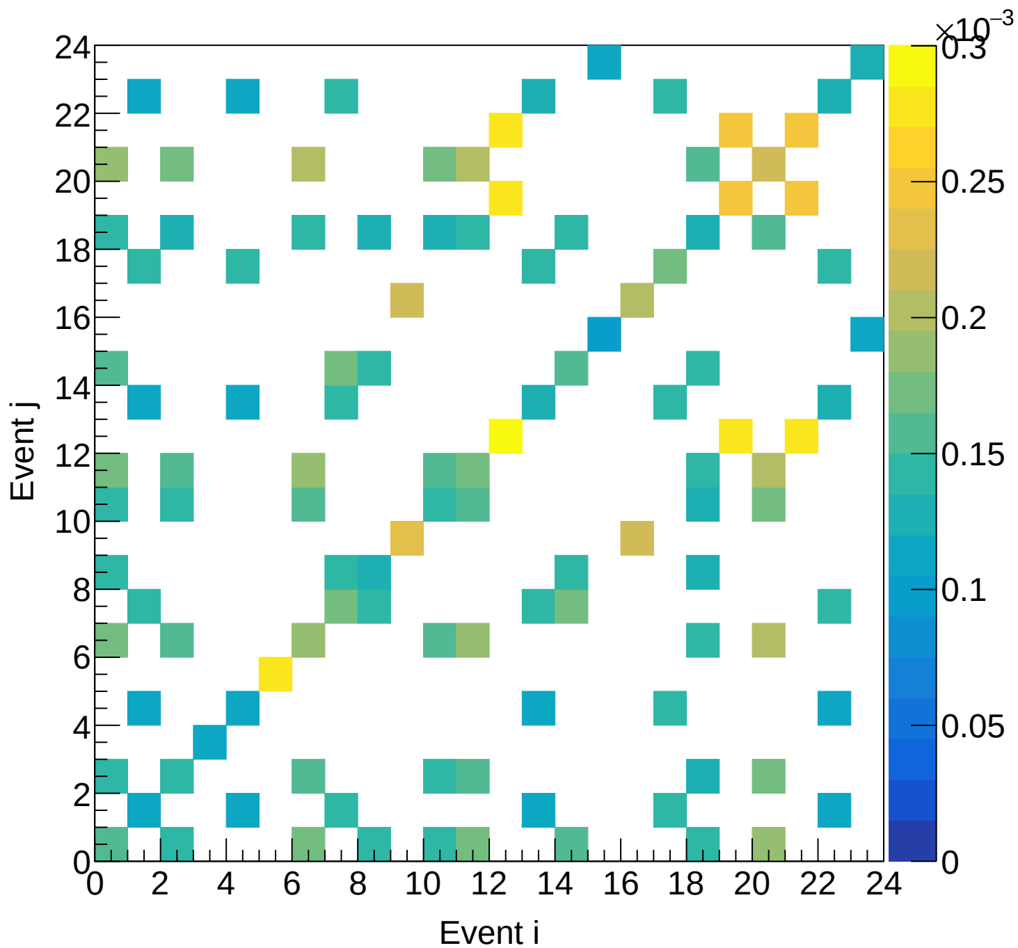
LD2 (mix) Covariance | M: [3.9, 4.2] xF: [0.75, 0.80)
