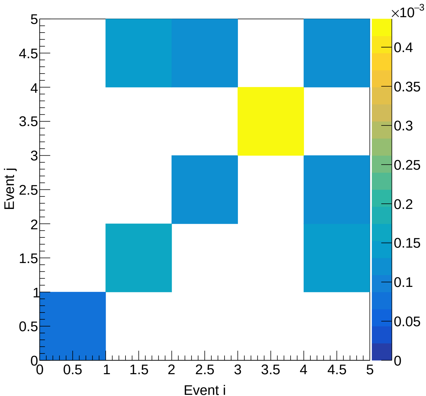
LD2 (mix) Covariance | M: [4.2, 4.5) xF: [0.75, 0.80)
