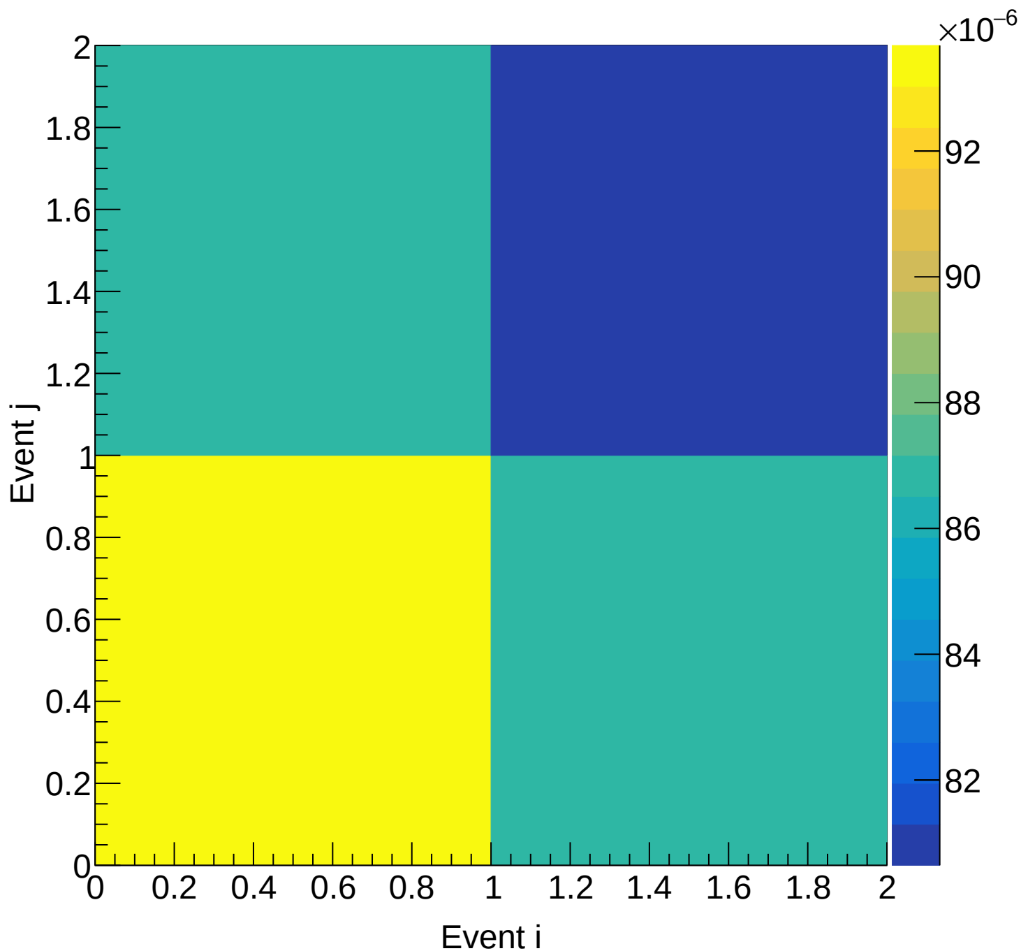
LD2 (mix) Covariance | M: [4.5, 4.8) xF: [0.75, 0.80)
