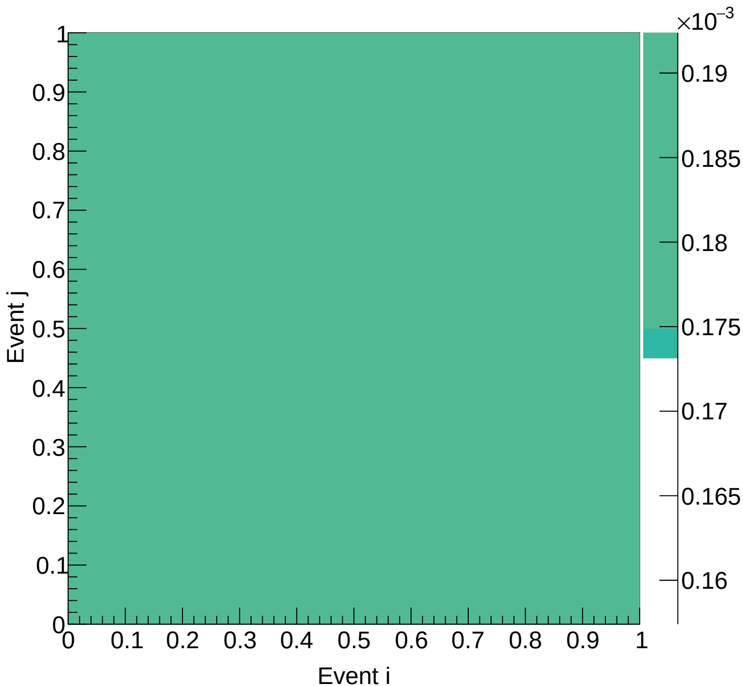
LD2 (mix) Covariance | M: [5.1, 5.4) xF: [0.75, 0.80)
