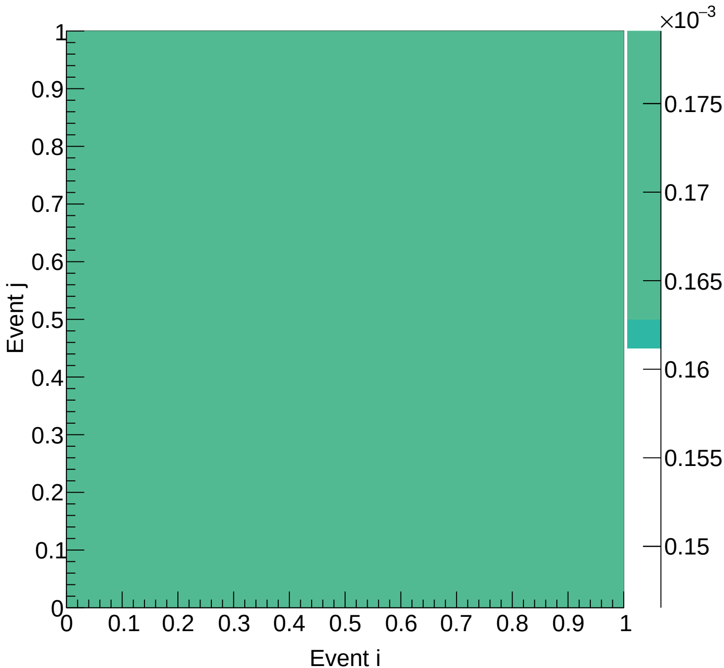
LD2 (mix) Covariance | M: [5.7, 6.0] xF: [0.75, 0.80)
