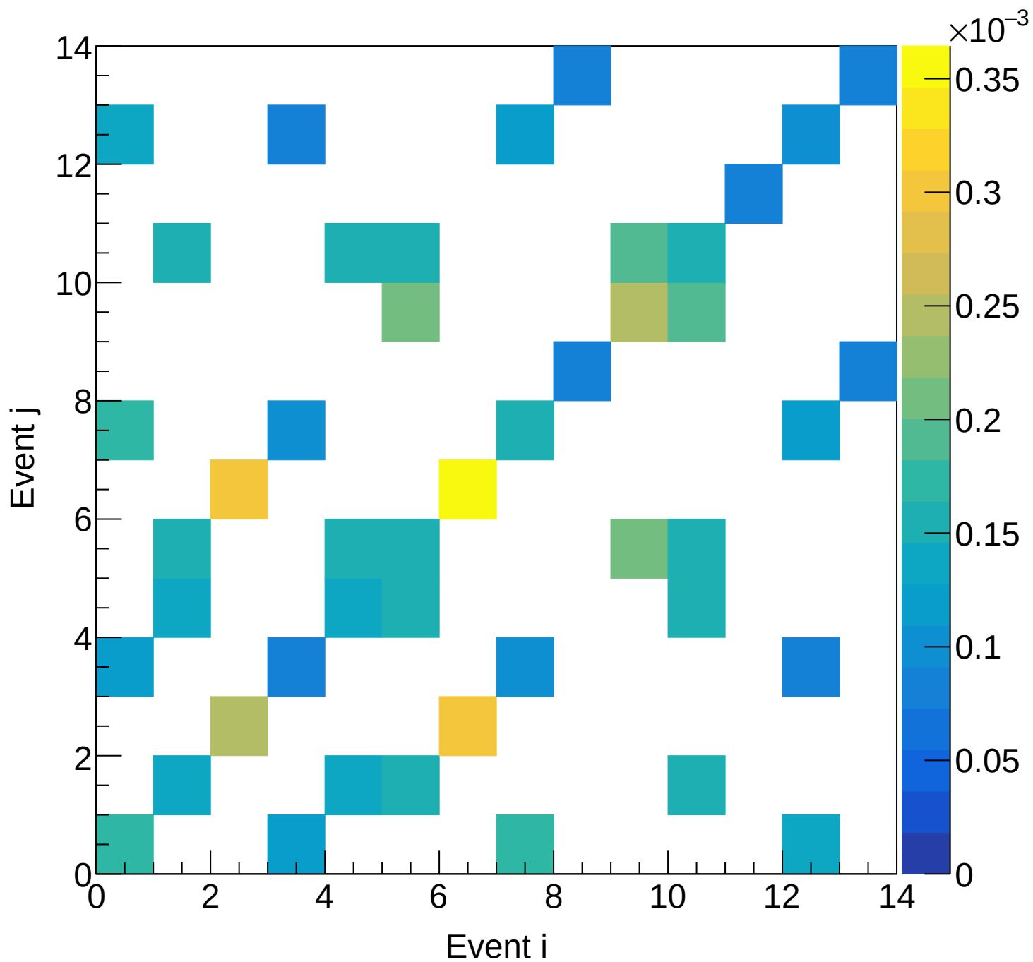
LD2 (mix) Covariance | M: [3.9, 4.2) xF: [0.80, 0.85)
