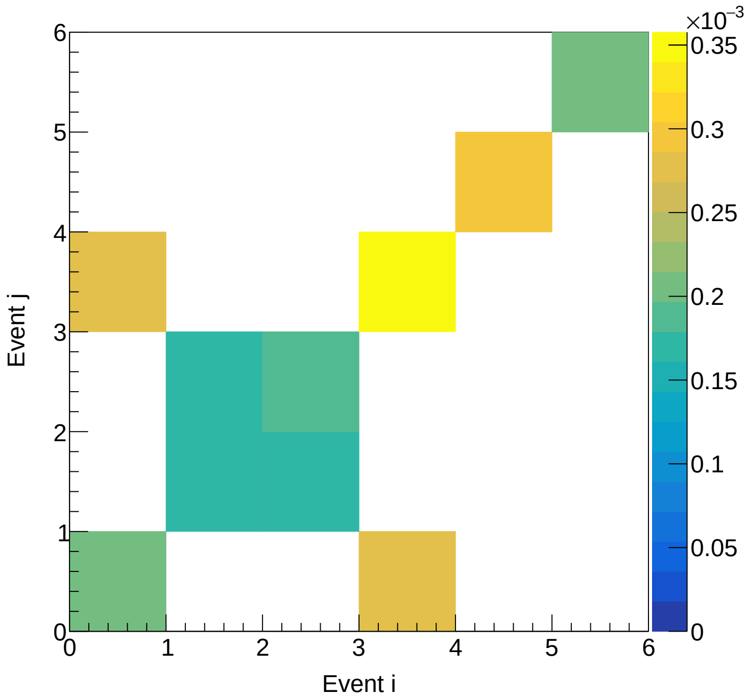
LD2 (mix) Covariance | M: [4.2, 4.5) xF: [0.80, 0.85)
