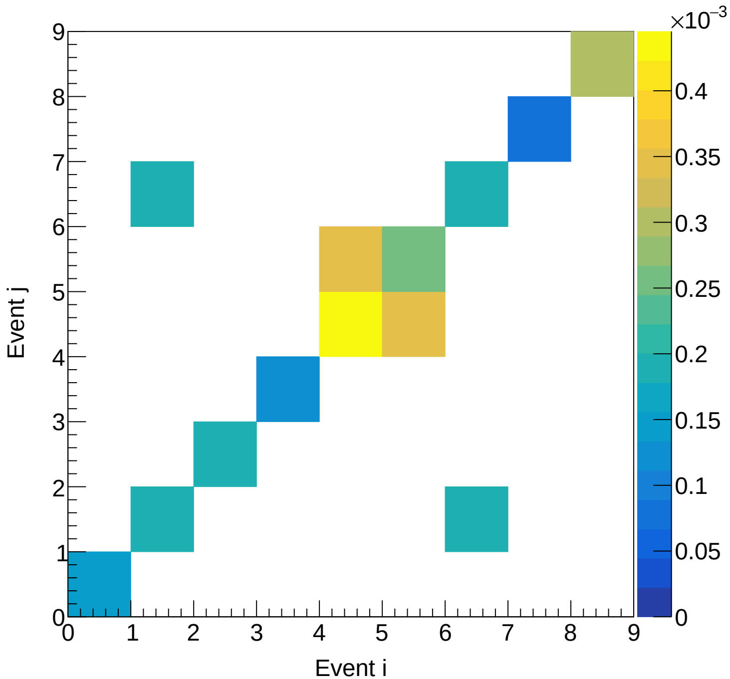
LD2 (mix) Covariance | M: [3.9, 4.2) xF: [0.85, 0.90)
