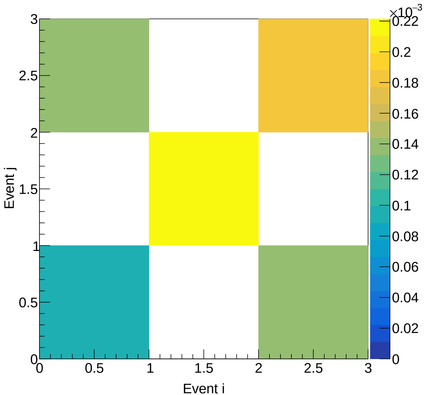
LD2 (mix) Covariance | M: [4.5, 4.8) xF: [0.85, 0.90)
