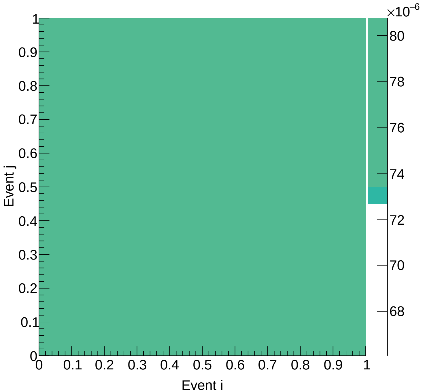
LD2 (mix) Covariance | M: [4.8, 5.1) xF: [0.85, 0.90)
