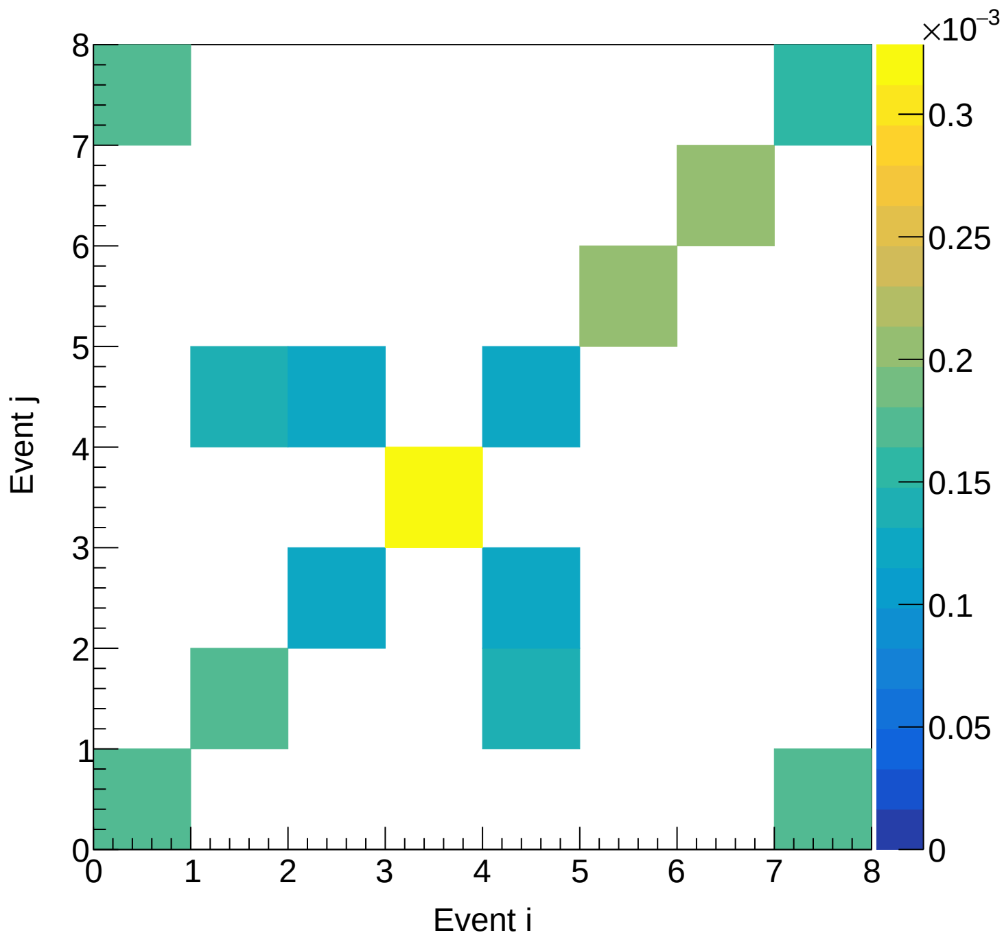
LD2 (mix) Covariance | M: [3.9, 4.2) xF: [0.90, 0.95)
