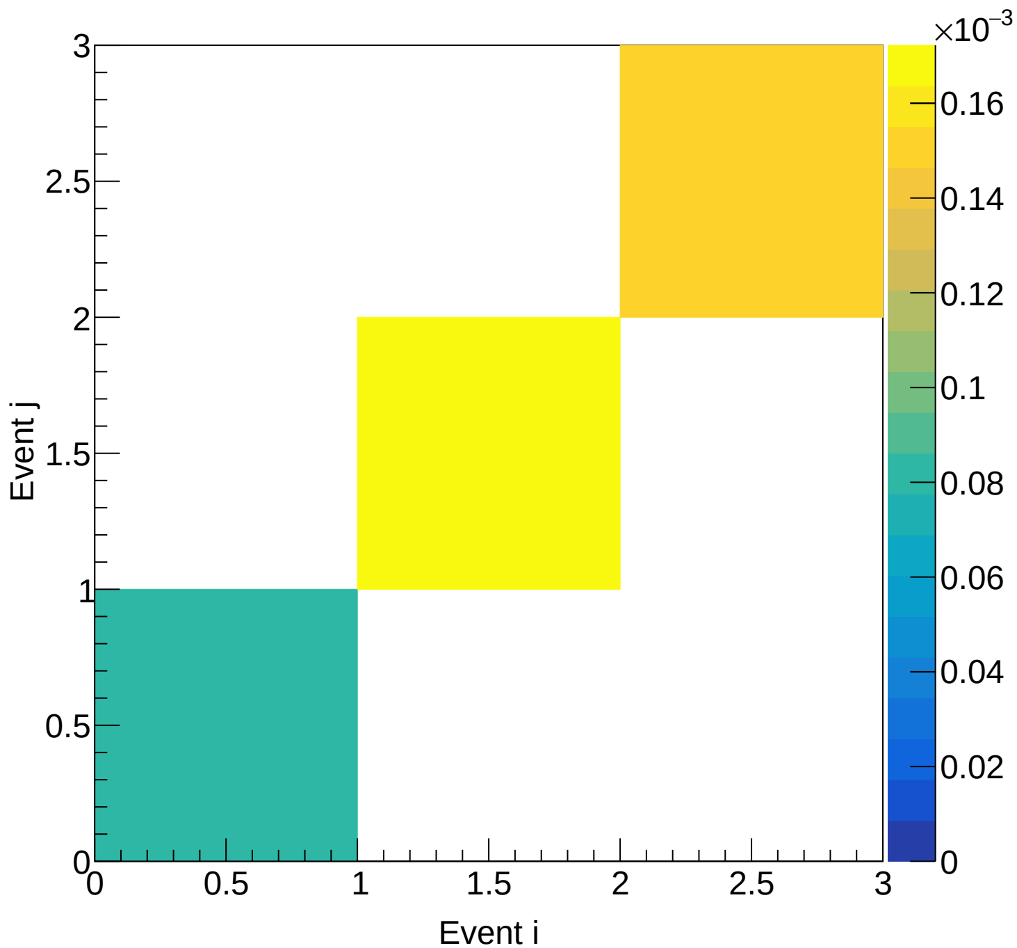
LD2 (mix) Covariance | M: [4.2, 4.5) xF: [0.90, 0.95)
