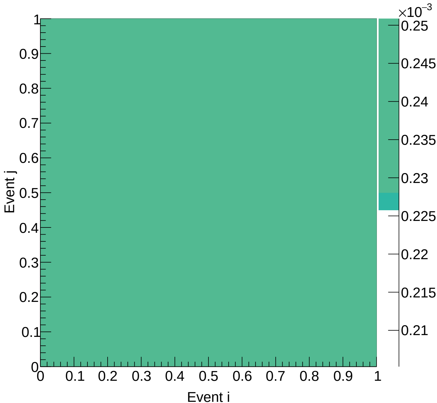
LD2 (mix) Covariance | M: [6.0, 6.3) xF: [0.90, 0.95)
