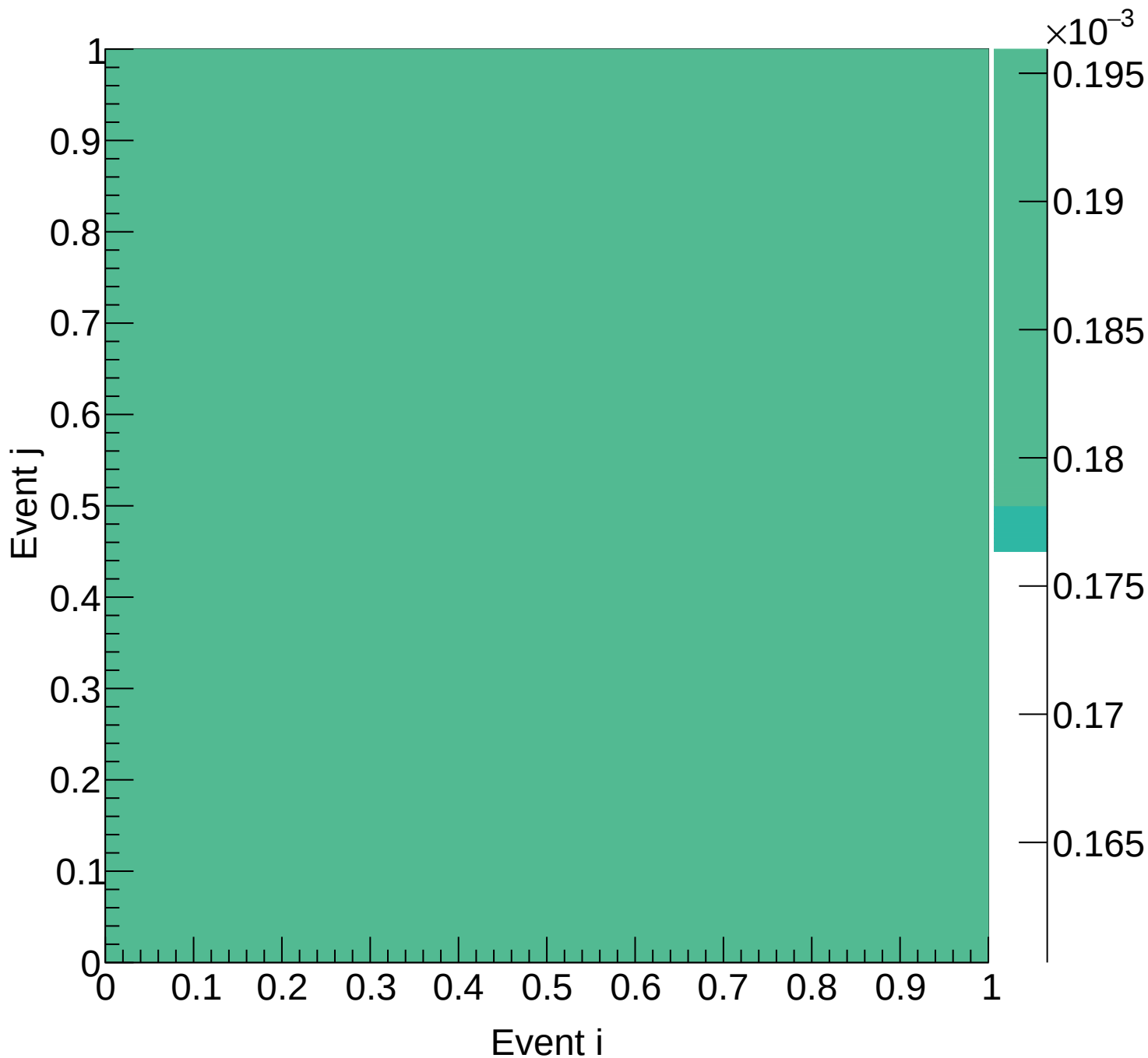
LD2 (mix) Covariance | M: [6.3, 6.6) xF: [0.00, 0.05)
