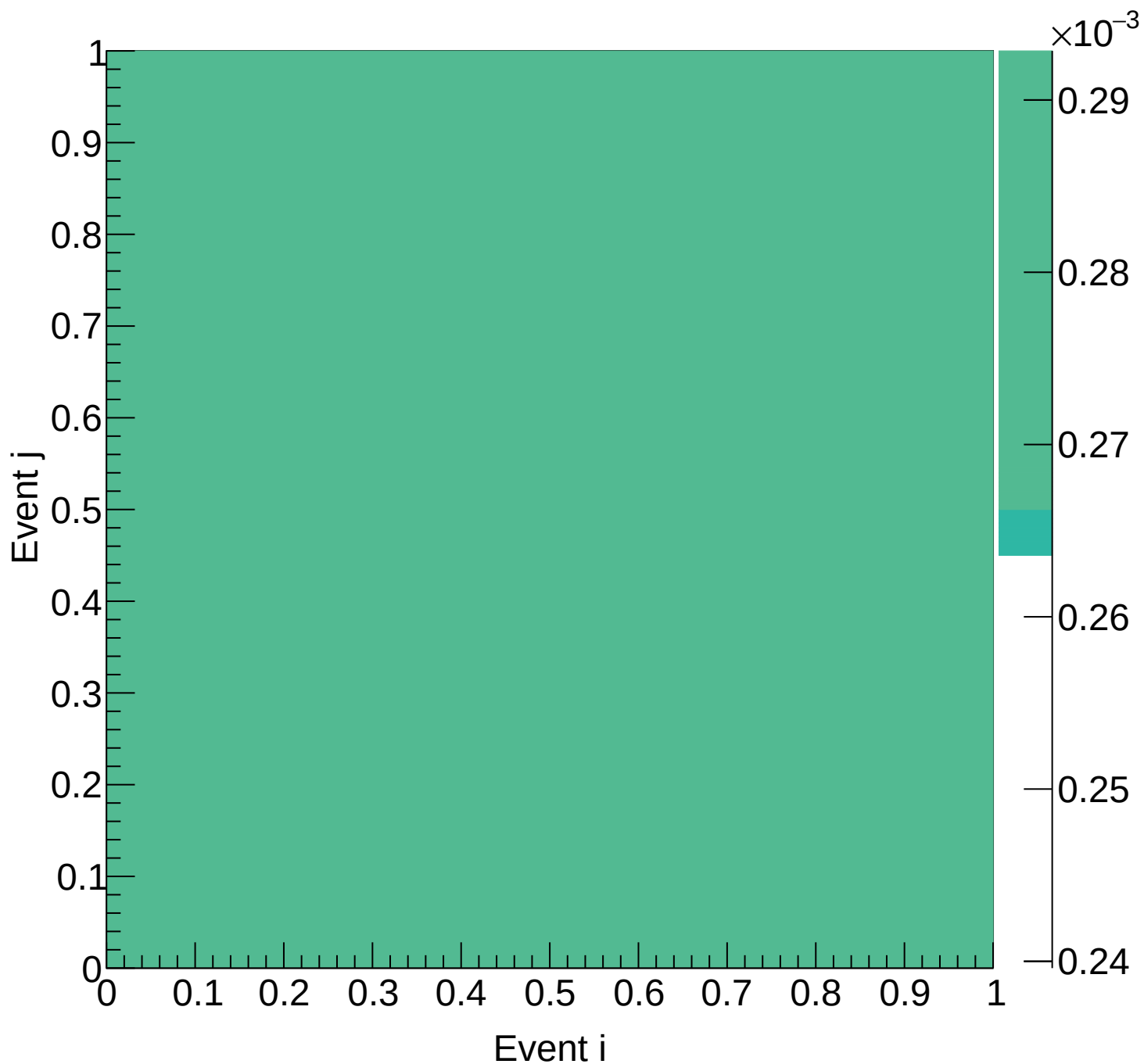
LD2 (mix) Covariance | M: [4.2, 4.5) xF: [0.05, 0.10)
