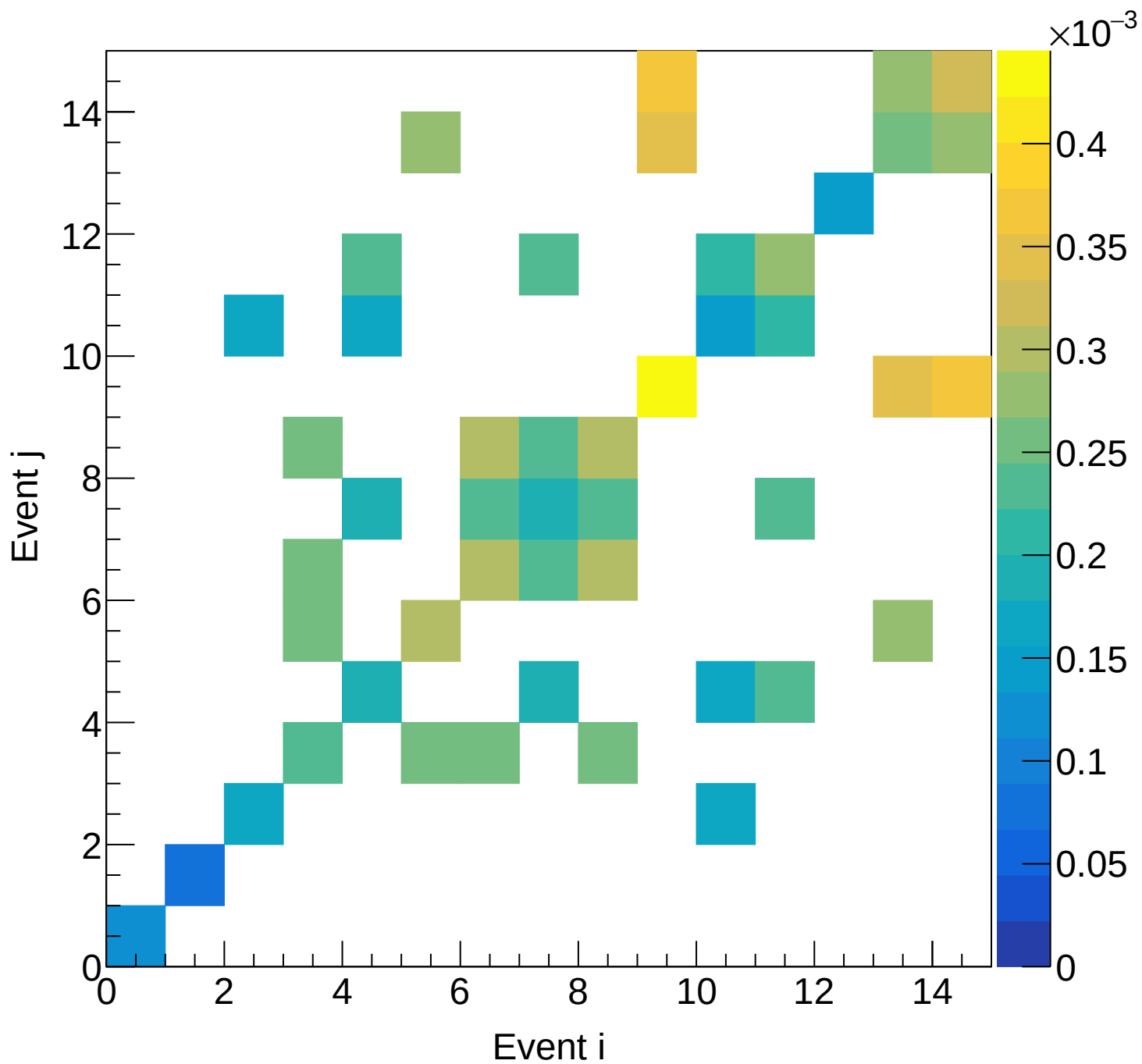
LD2 (mix) Covariance | M: [5.4, 5.7] xF: [0.05, 0.10)
