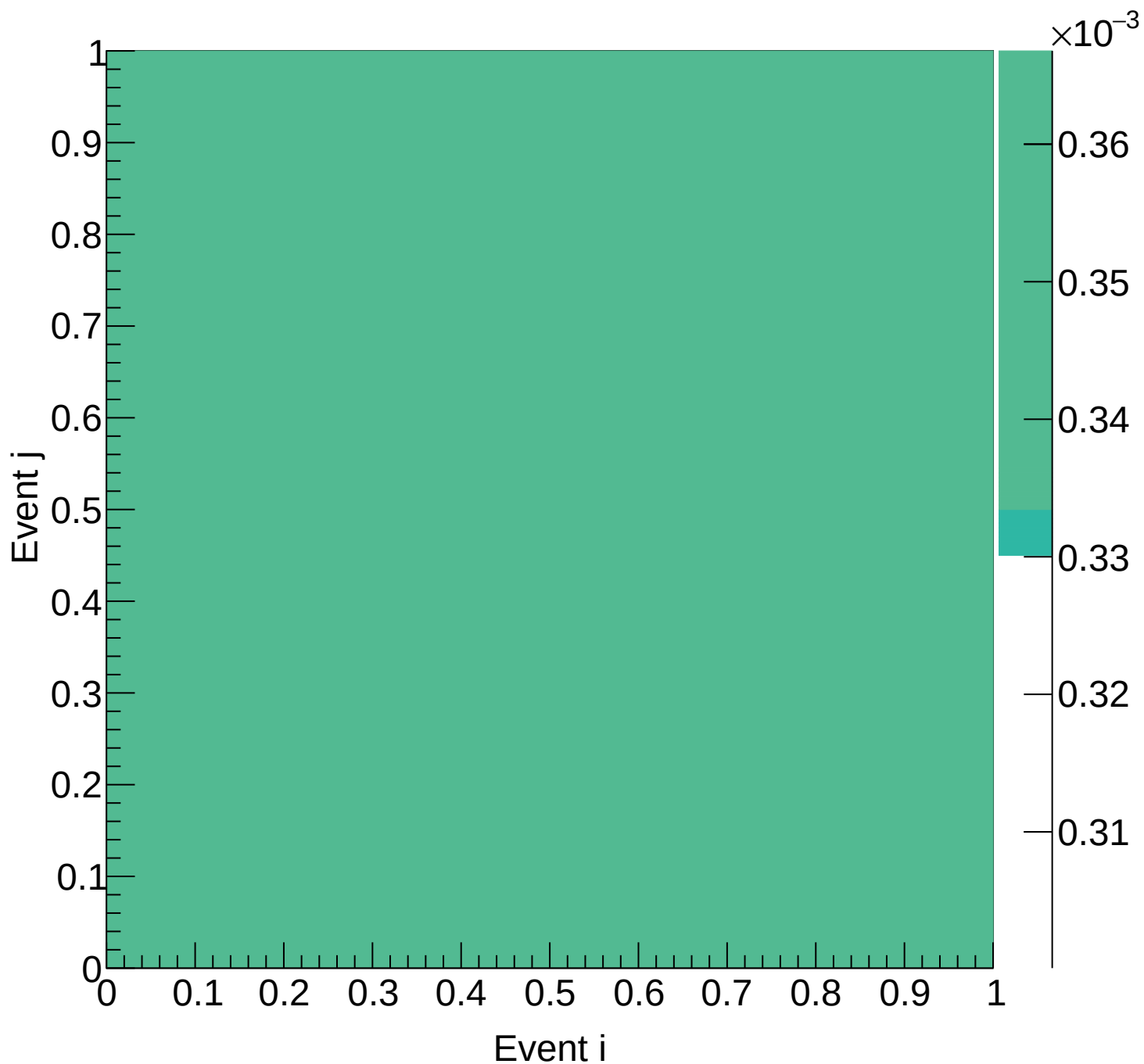
LD2 (mix) Covariance | M: [6.9, 7.5) xF: [0.10, 0.15)
