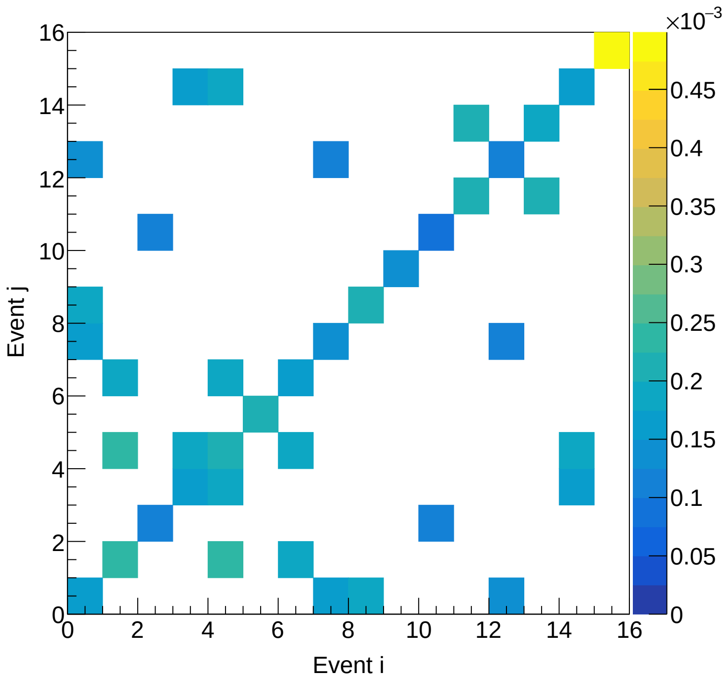
LD2 (mix) Covariance | M: [5.4, 5.7) xF: [0.10, 0.15)
