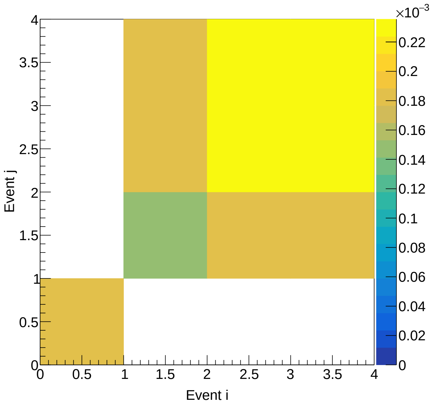
LD2 (mix) Covariance | M: [5.7, 6.0) xF: [0.10, 0.15)
