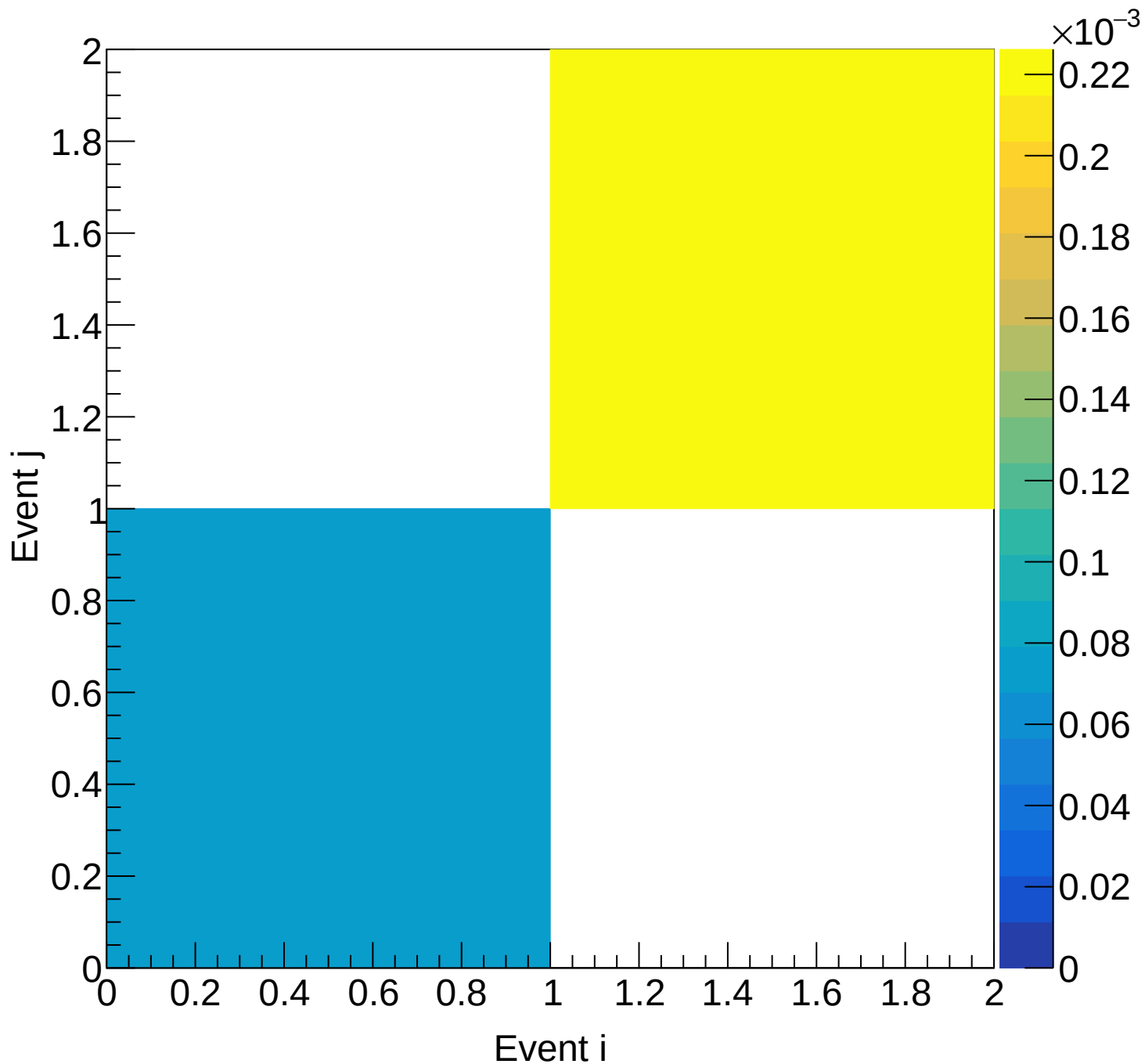
LD2 (mix) Covariance | M: [6.3, 6.6] xF: [0.10, 0.15)
