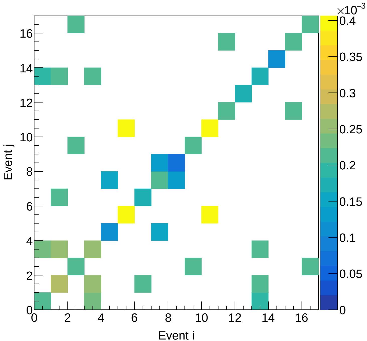
LD2 (mix) Covariance | M: [5.4, 5.7) xF: [0.15, 0.20)
