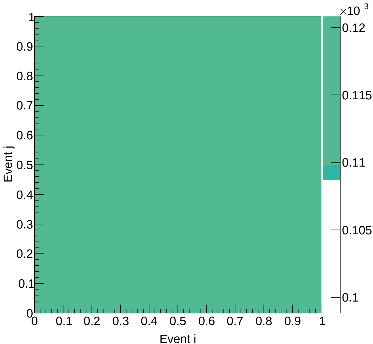
LD2 (mix) Covariance | M: [6.3, 6.6] xF: [0.15, 0.20)
