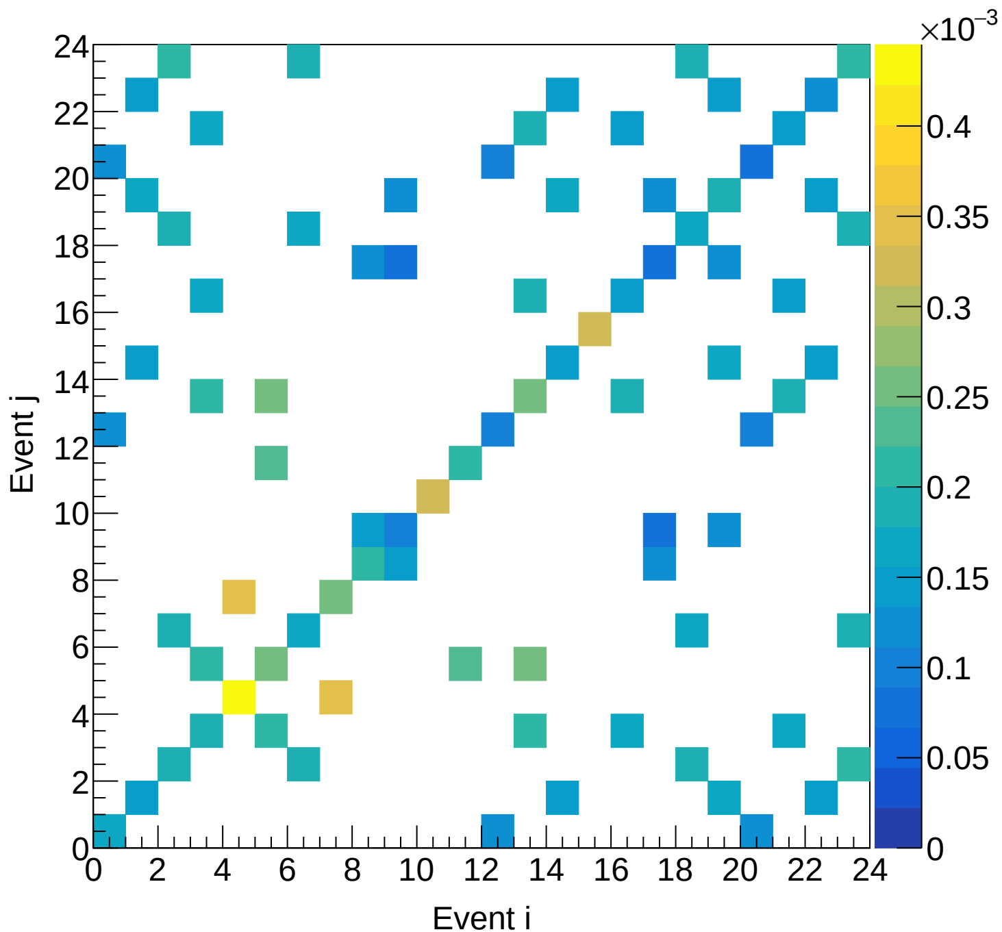
LD2 (mix) Covariance | M: [3.9, 4.2) xF: [0.20, 0.25)
