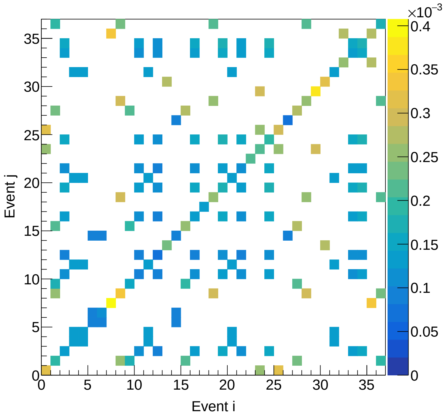
LD2 (mix) Covariance | M: [4.2, 4.5) xF: [0.20, 0.25)
