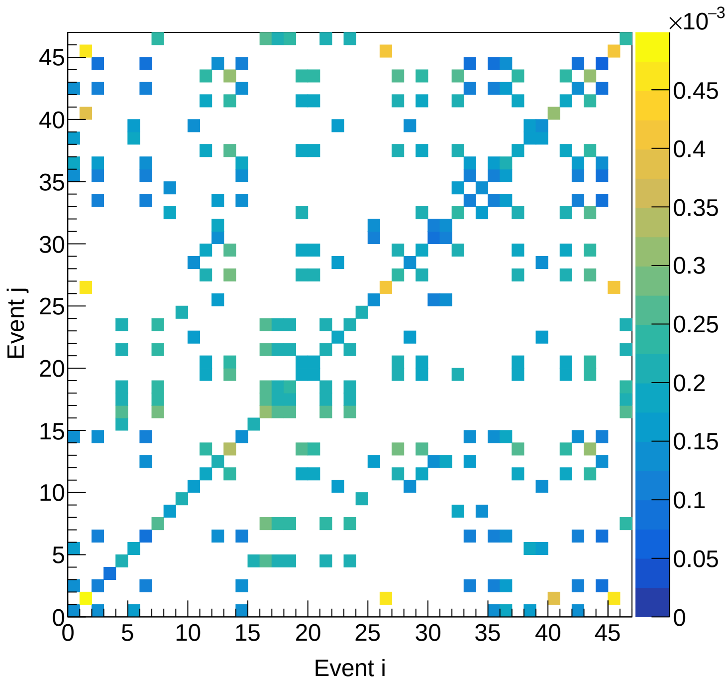
LD2 (mix) Covariance | M: [4.5, 4.8) xF: [0.20, 0.25)
