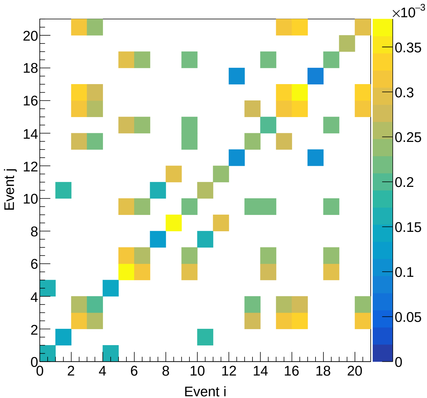
LD2 (mix) Covariance | M: [4.8, 5.1) xF: [0.20, 0.25)
