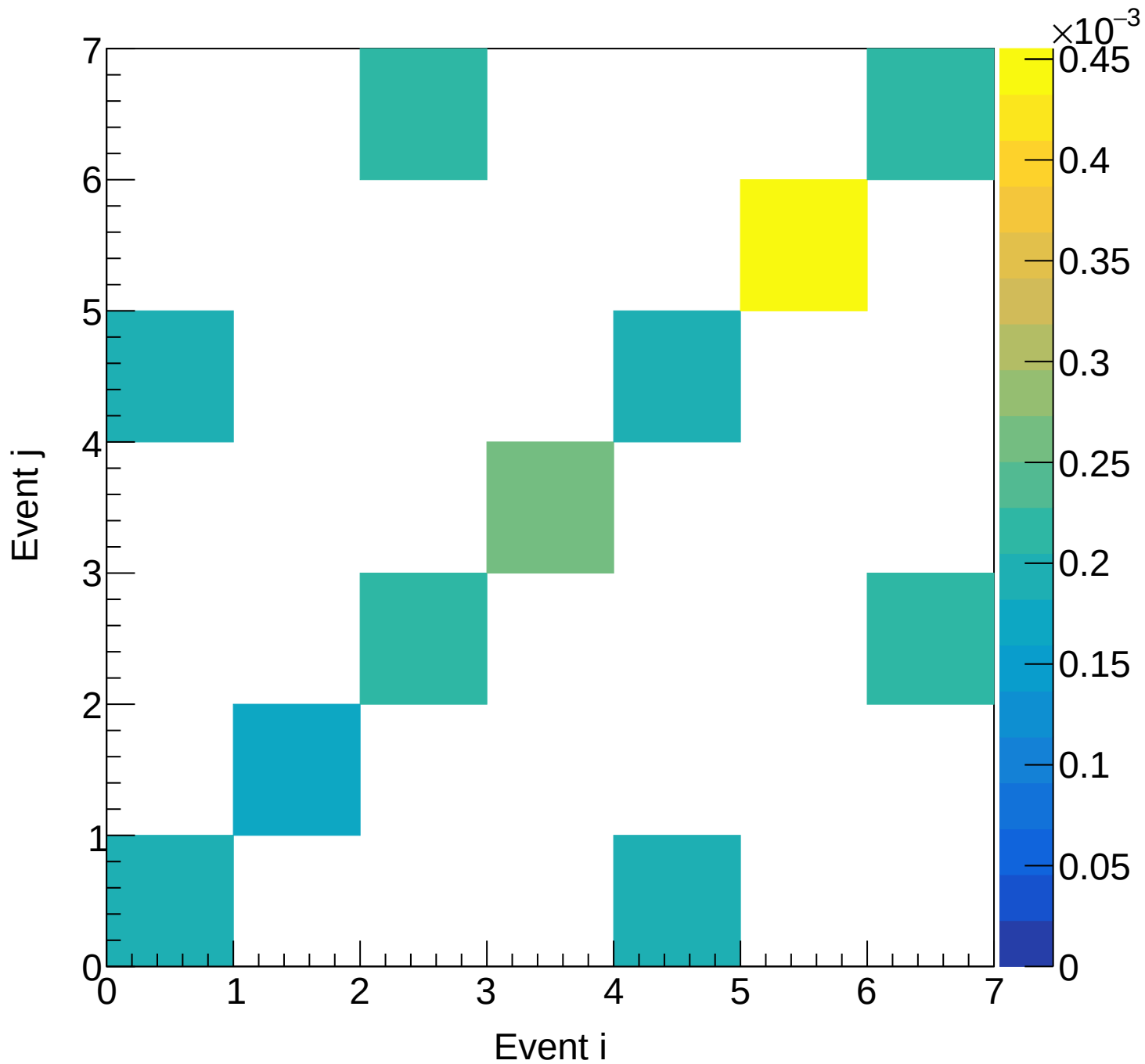
LD2 (mix) Covariance | M: [5.4, 5.7) xF: [0.20, 0.25)
