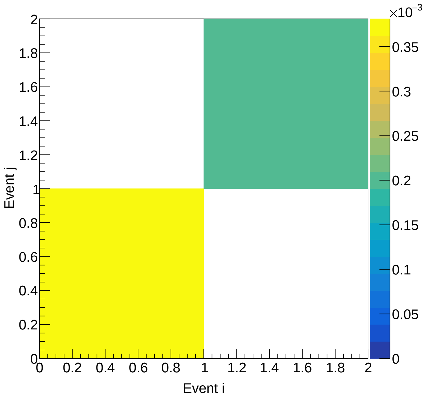
LD2 (mix) Covariance | M: [6.0, 6.3) xF: [0.20, 0.25)
