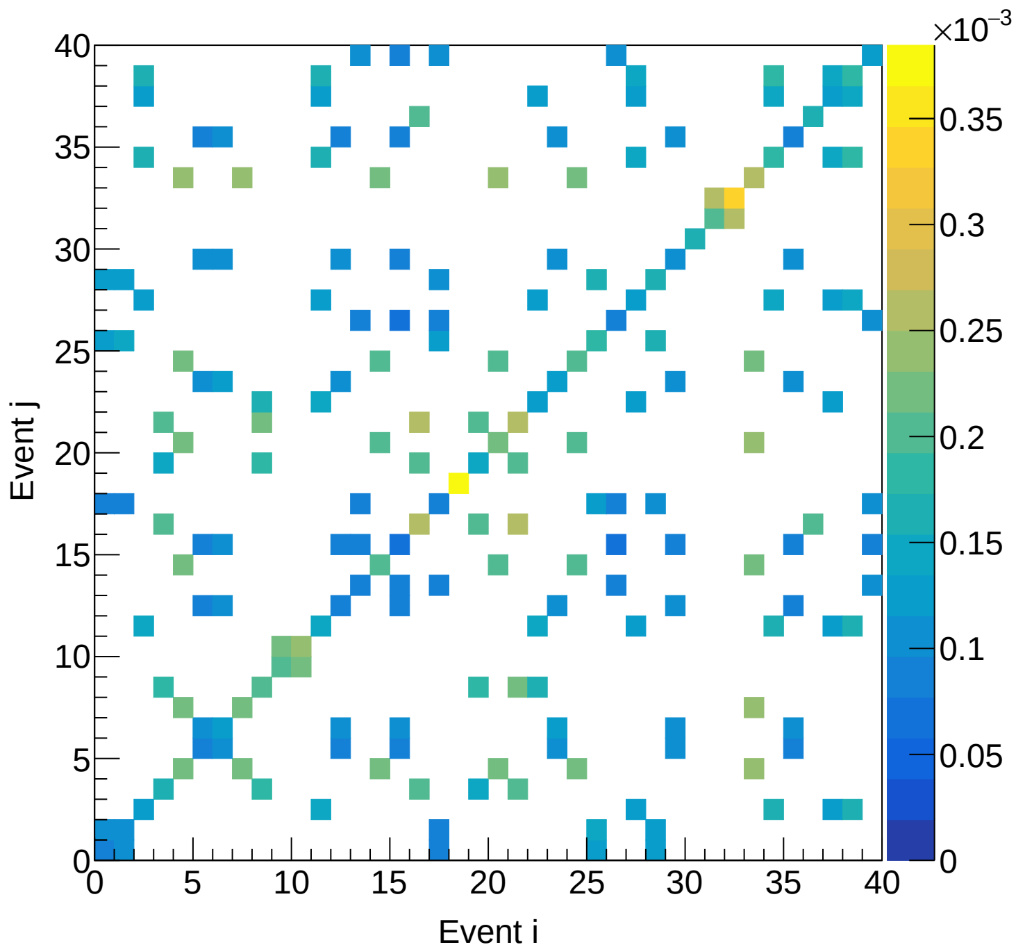
LD2 (mix) Covariance | M: [3.9, 4.2) xF: [0.25, 0.30)
