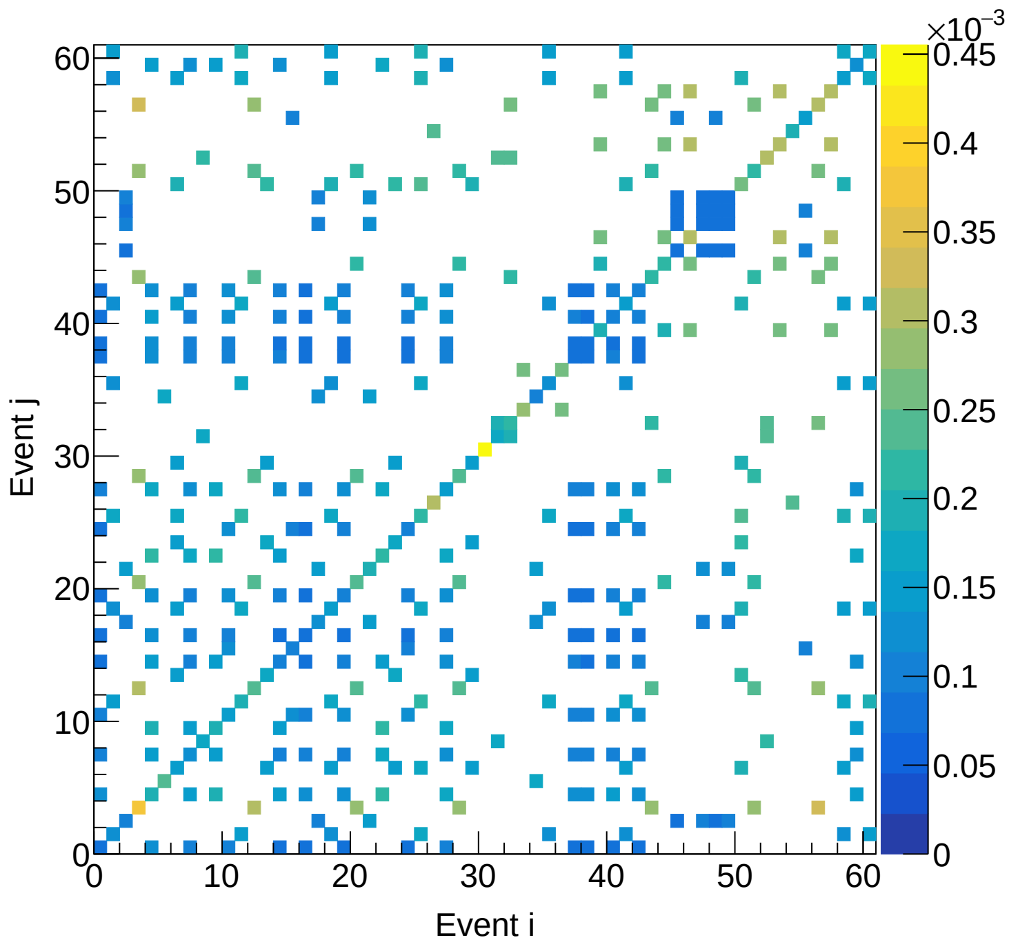
LD2 (mix) Covariance | M: [4.2, 4.5) xF: [0.25, 0.30)
