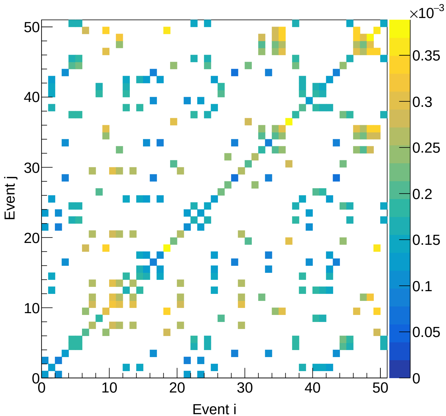
LD2 (mix) Covariance | M: [4.5, 4.8) xF: [0.25, 0.30)
