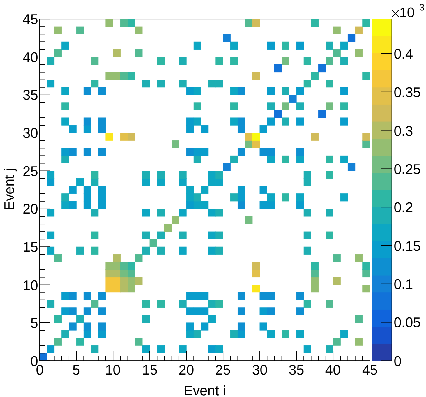
LD2 (mix) Covariance | M: [4.8, 5.1) xF: [0.25, 0.30)
