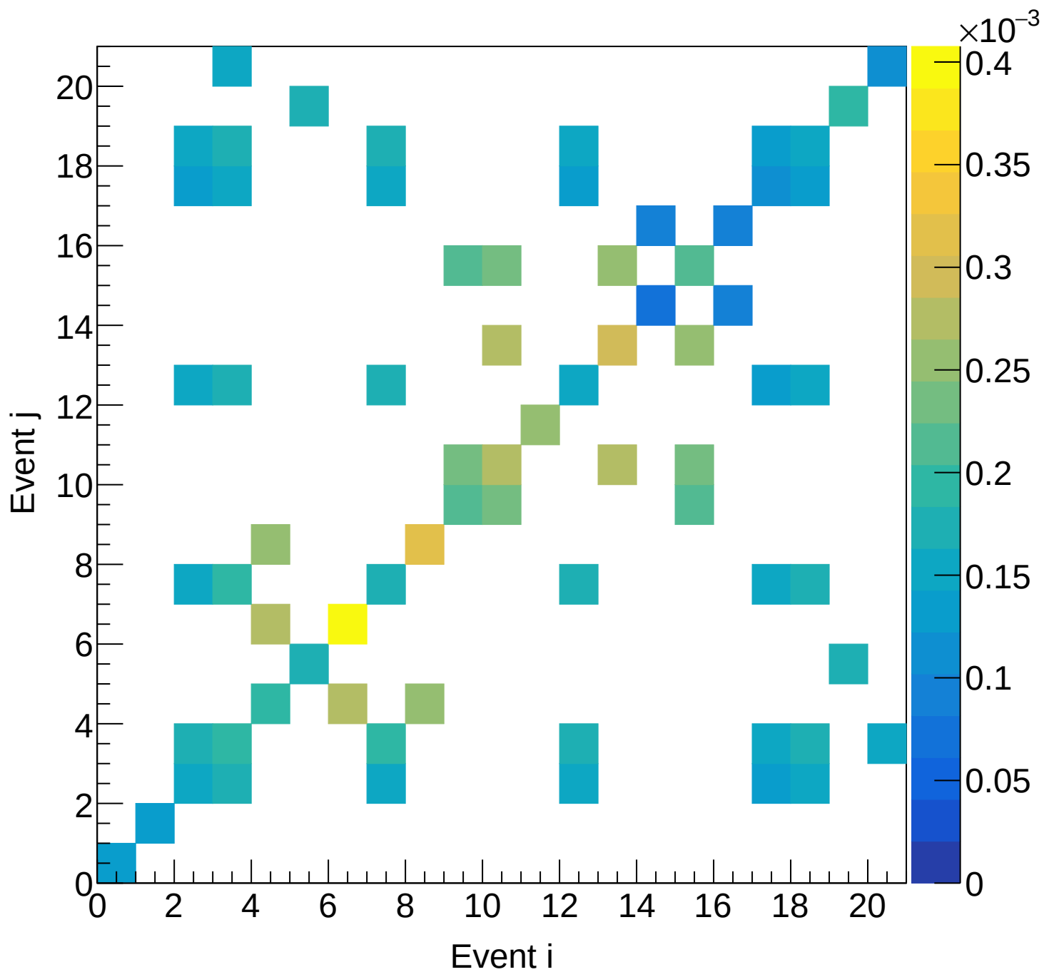
LD2 (mix) Covariance | M: [5.1, 5.4) xF: [0.25, 0.30)
