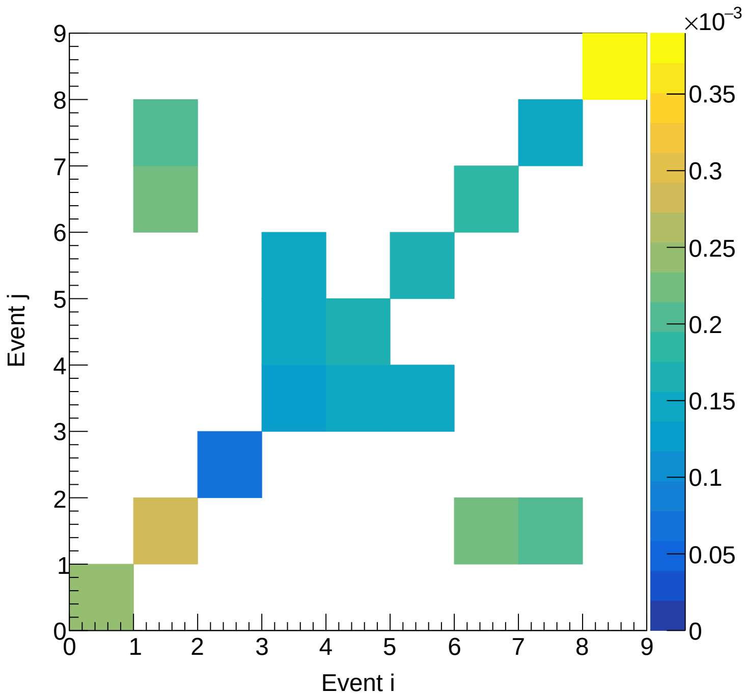
LD2 (mix) Covariance | M: [5.4, 5.7] xF: [0.25, 0.30)
