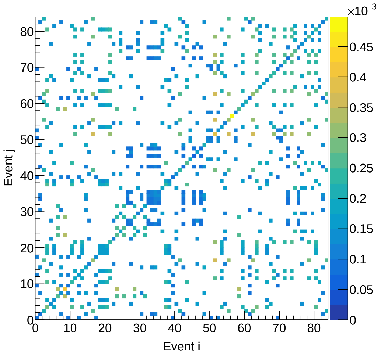
LD2 (mix) Covariance | M: [4.2, 4.5) xF: [0.30, 0.35)
