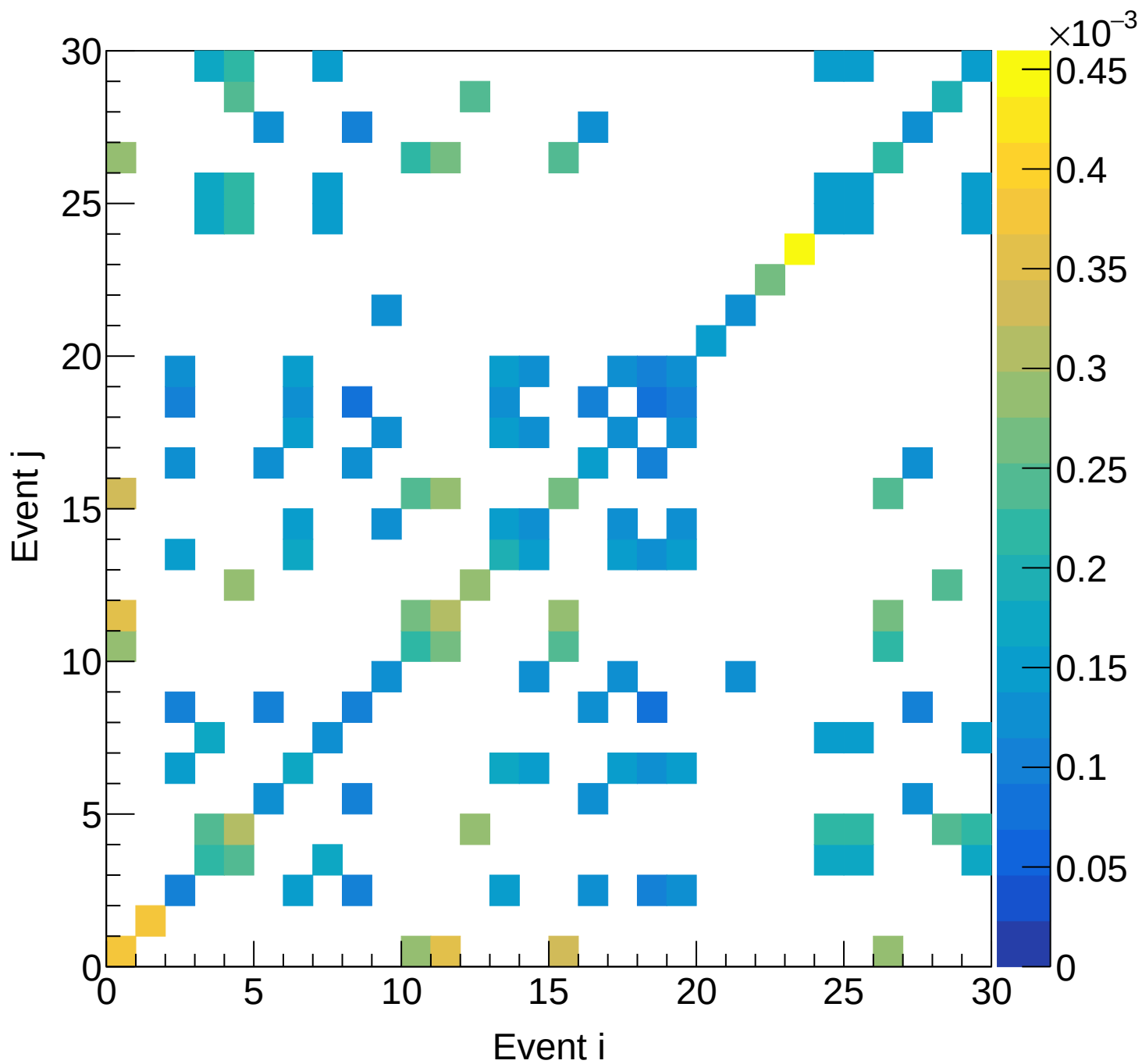
LD2 (mix) Covariance | M: [4.8, 5.1) xF: [0.30, 0.35)
