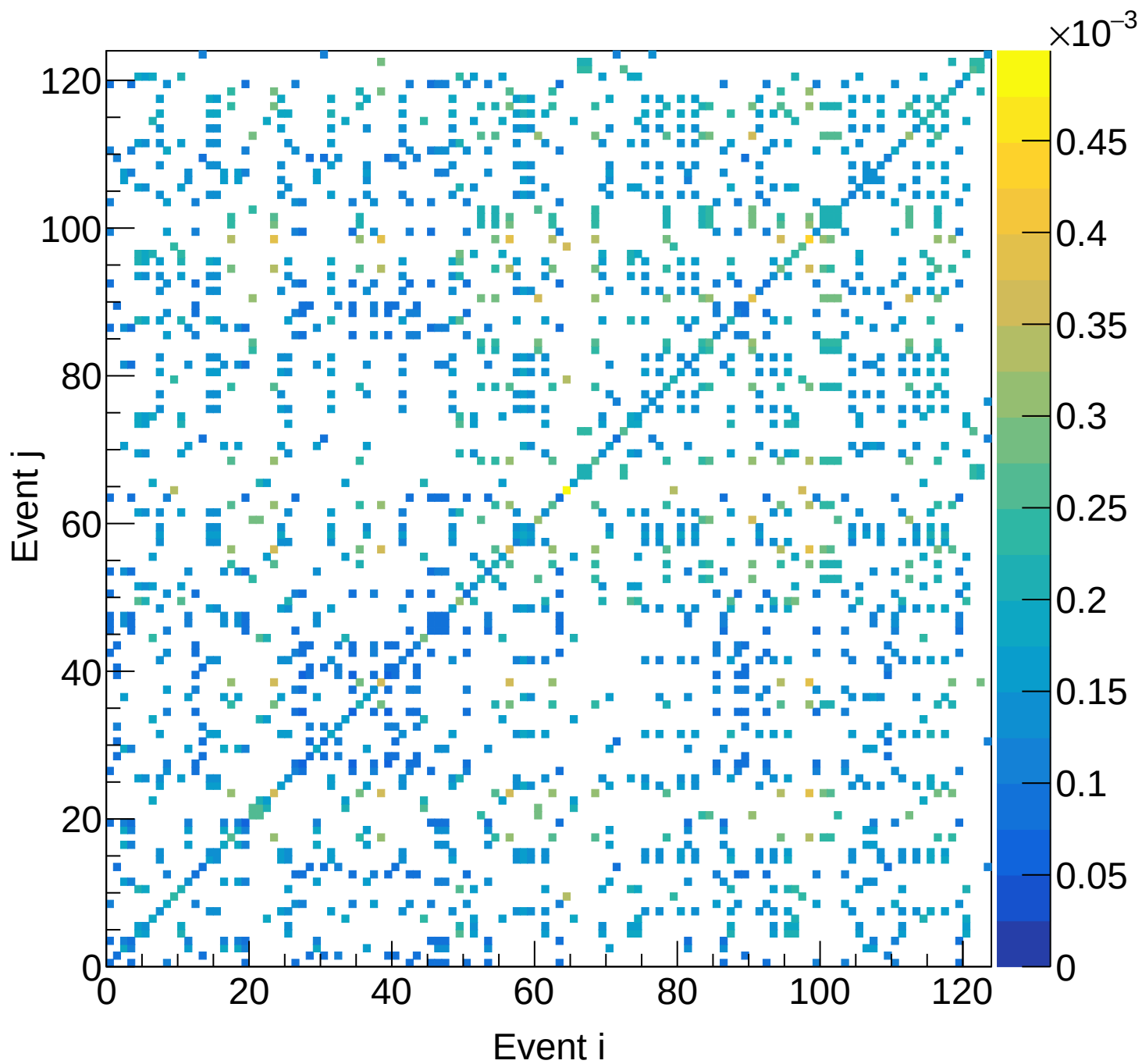
LD2 (mix) Covariance | M: [3.9, 4.2) xF: [0.35, 0.40)
