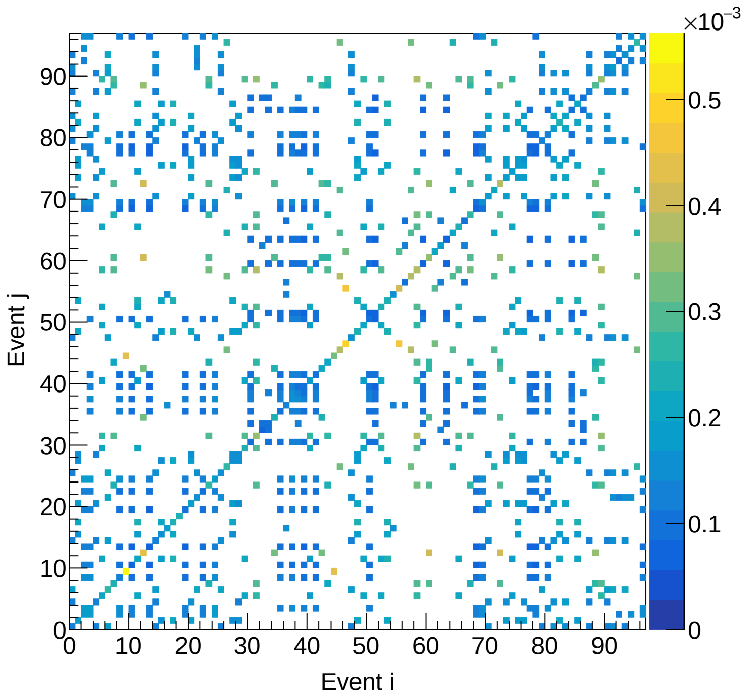
LD2 (mix) Covariance | M: [4.2, 4.5) xF: [0.35, 0.40)
