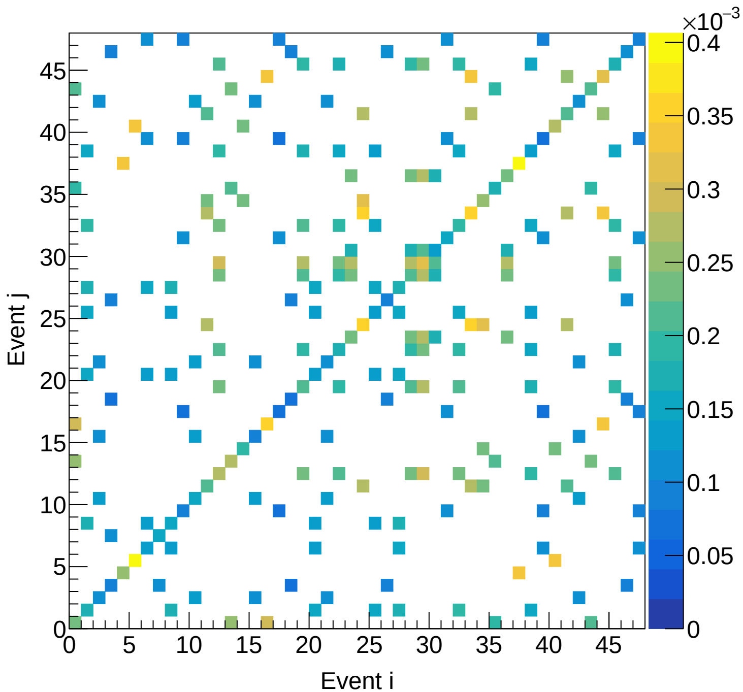
LD2 (mix) Covariance | M: [4.5, 4.8) xF: [0.35, 0.40)
