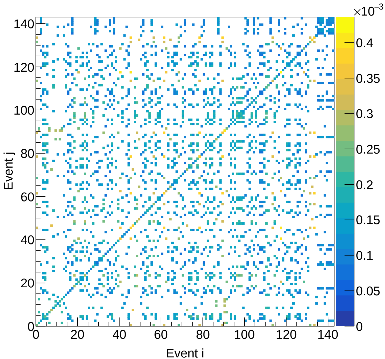
LD2 (mix) Covariance | M: [3.9, 4.2) xF: [0.40, 0.45)
