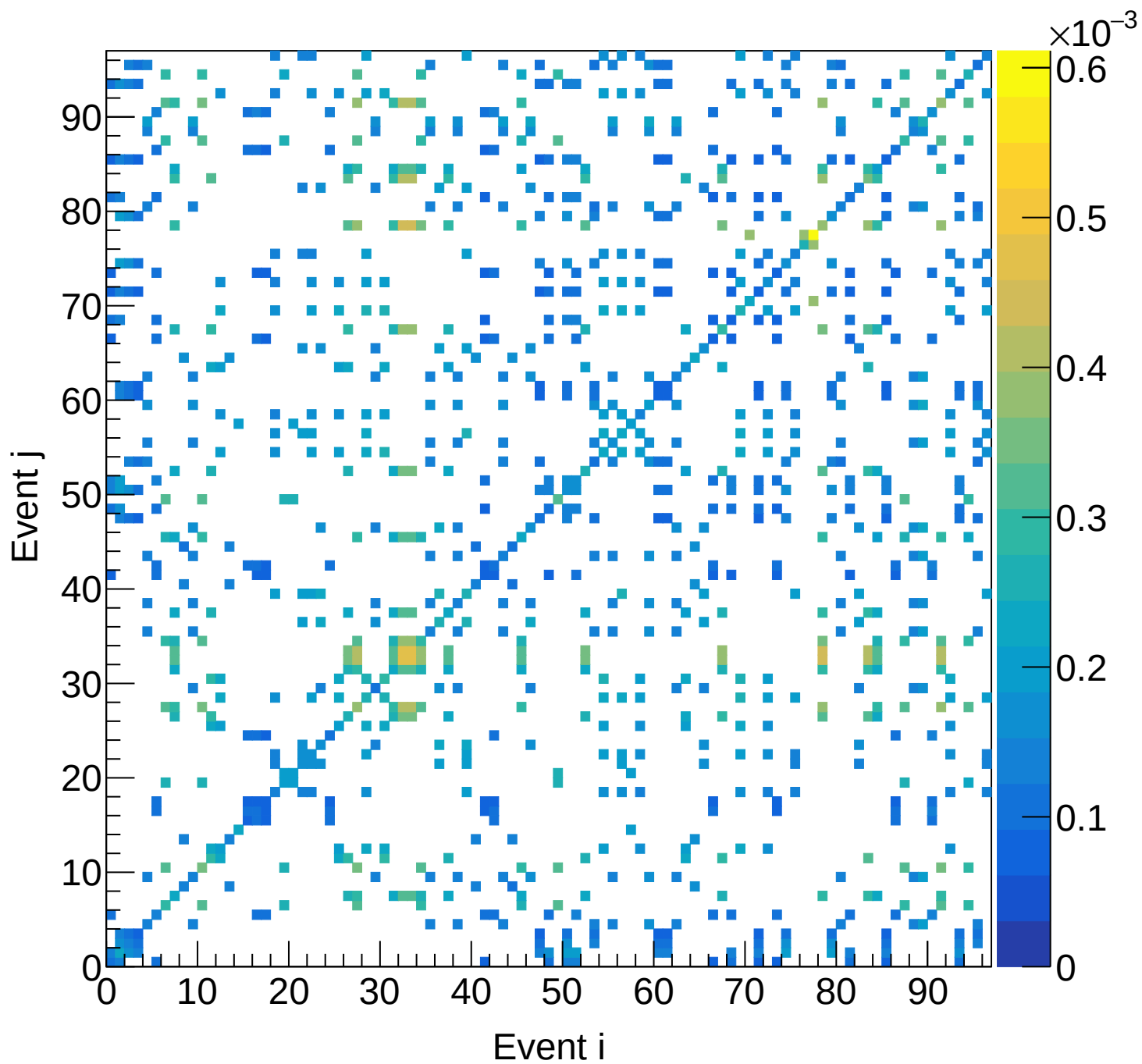
LD2 (mix) Covariance | M: [4.2, 4.5) xF: [0.40, 0.45)
