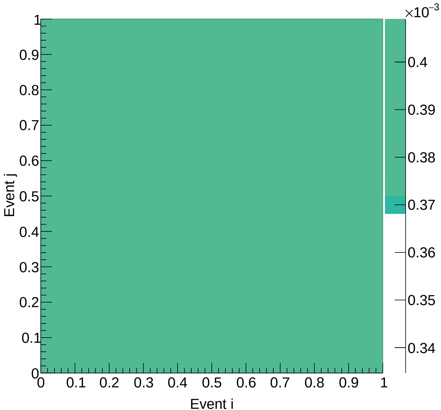
LD2 (mix) Covariance | M: [8.8, 10.0) xF: [0.40, 0.45)
