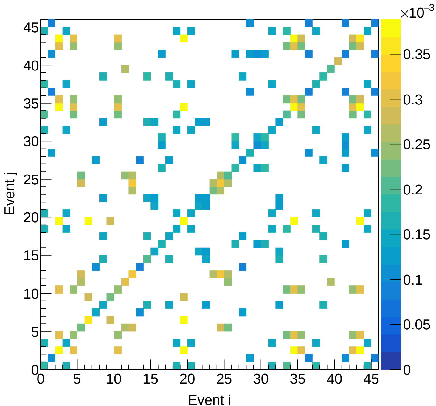
LD2 (mix) Covariance | M: [4.5, 4.8) xF: [0.40, 0.45)
