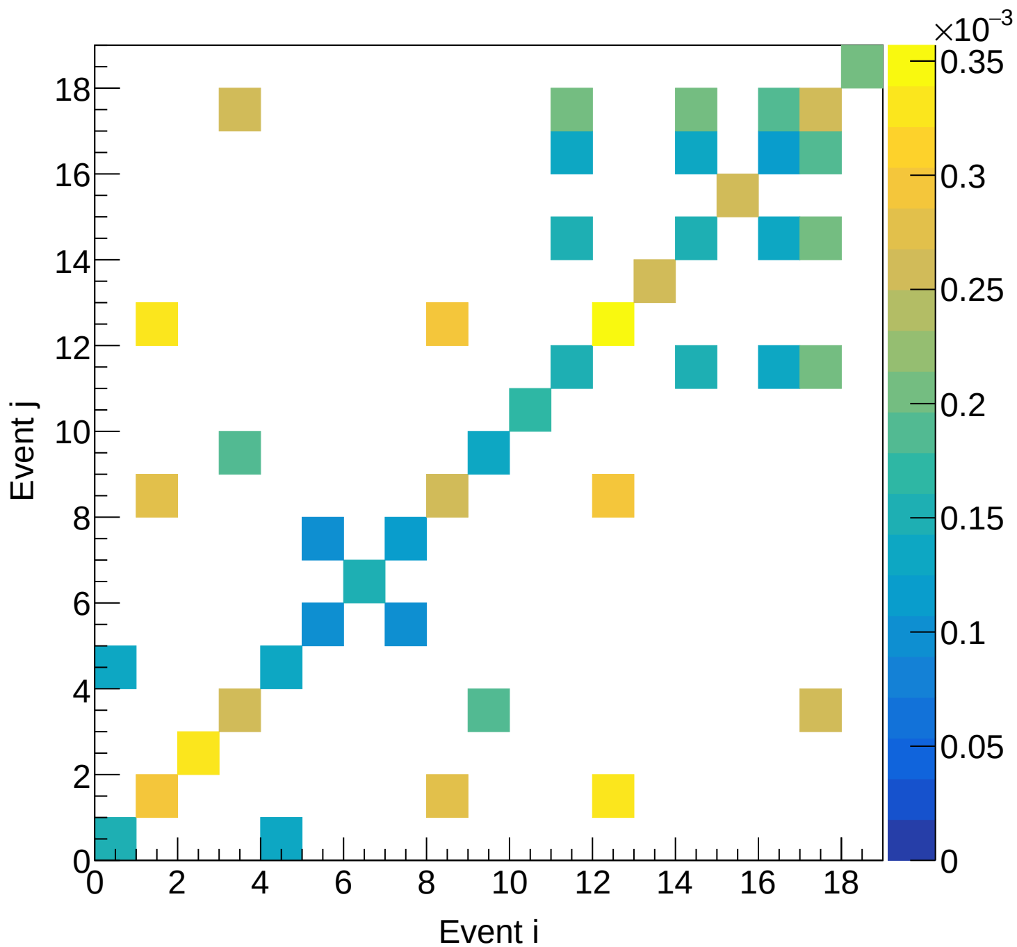
LD2 (mix) Covariance | M: [4.8, 5.1) xF: [0.40, 0.45)
