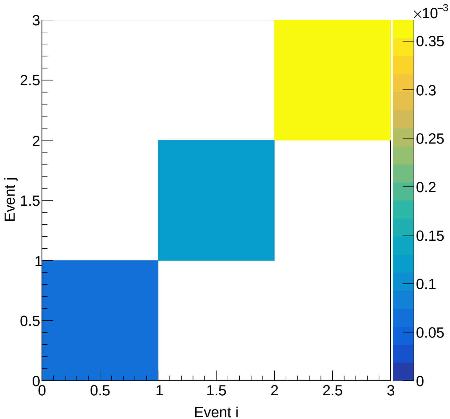
LD2 (mix) Covariance | M: [5.4, 5.7) xF: [0.40, 0.45)
