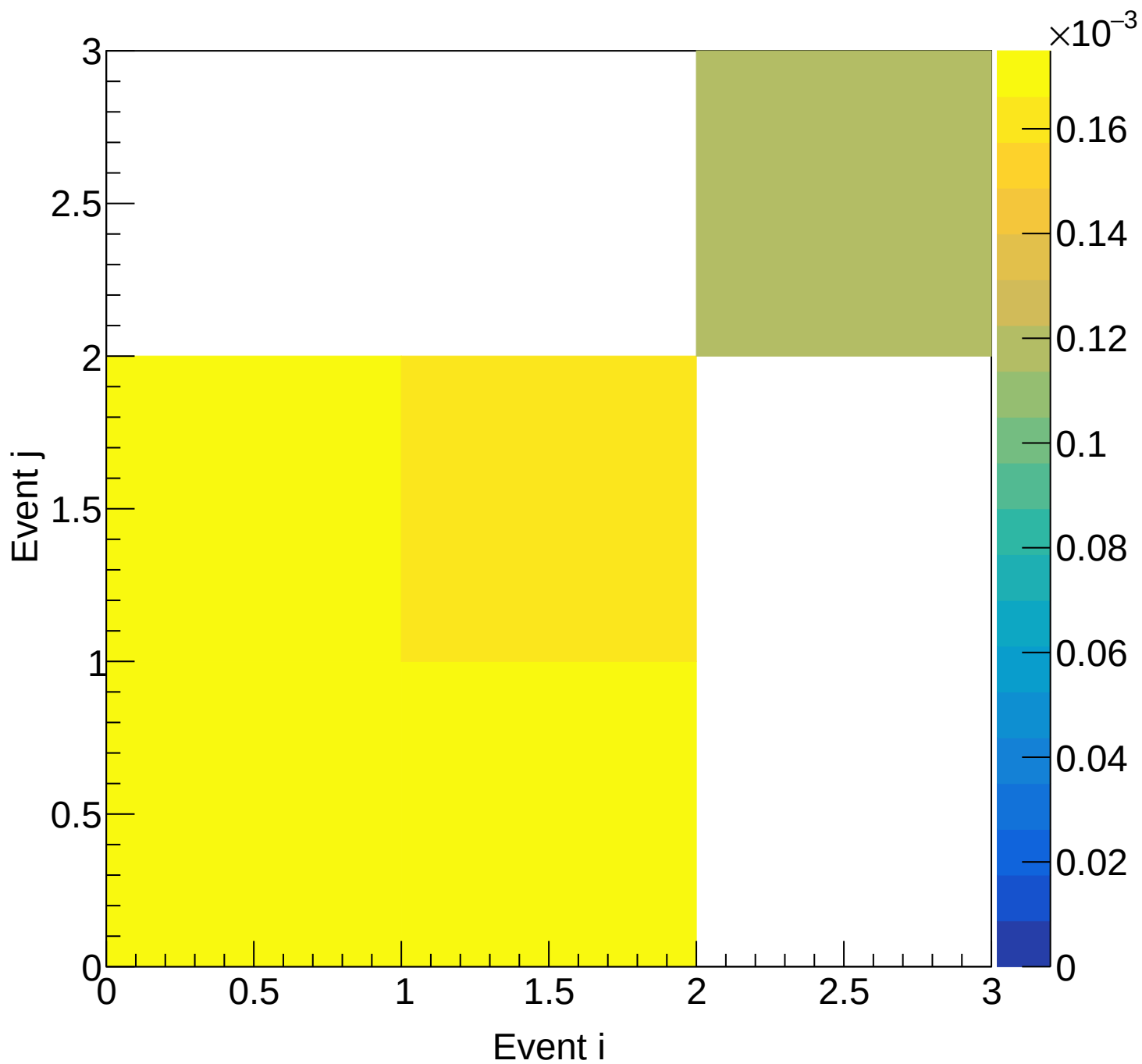
LD2 (mix) Covariance | M: [6.3, 6.6) xF: [0.40, 0.45)
