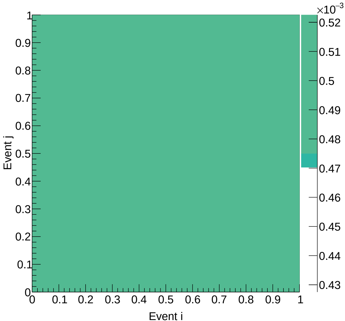
LD2 (mix) Covariance | M: [6.6, 6.9) xF: [0.40, 0.45)
