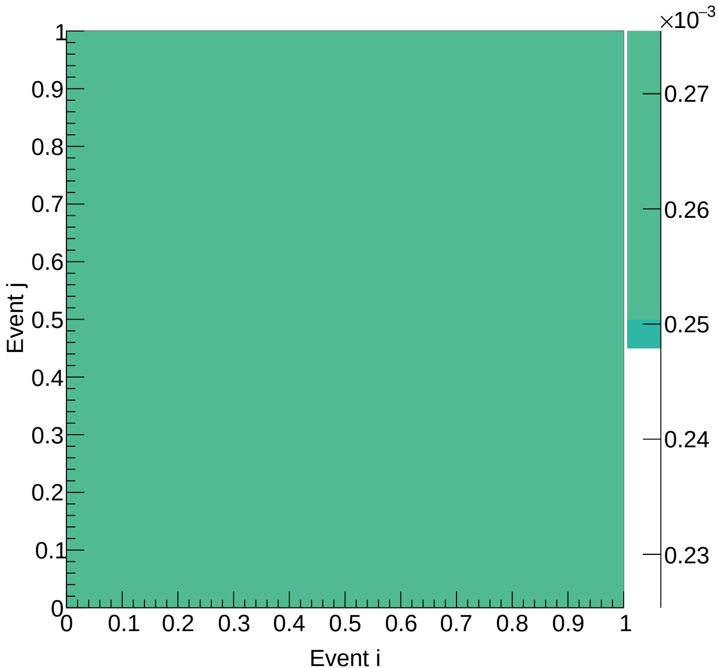
LD2 (total) Covariance | M: [7.5, 8.8) xF: [-0.05, 0.00)
