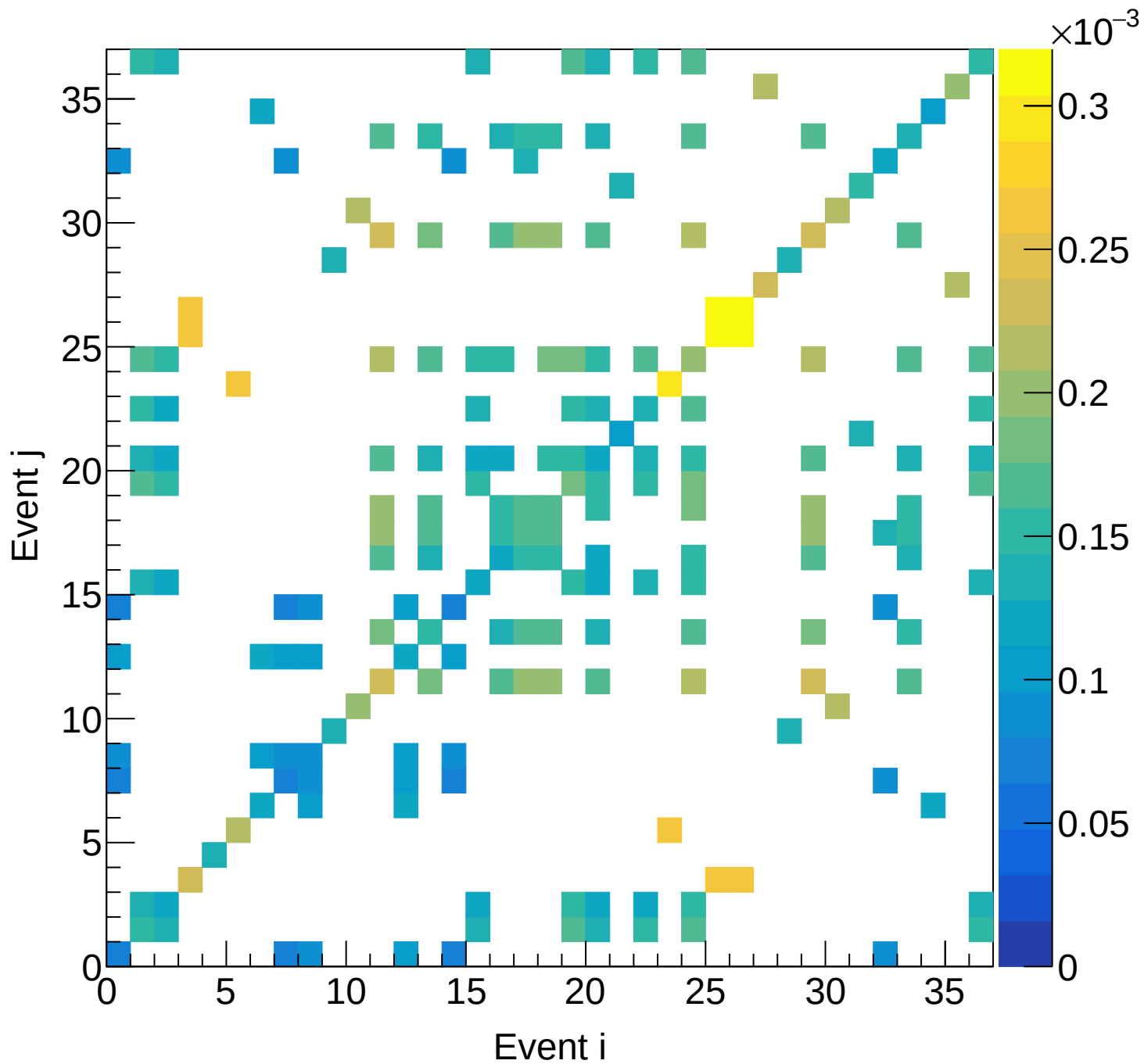
LD2 (total) Covariance | M: [5.4, 5.7) xF: [-0.05, 0.00)
