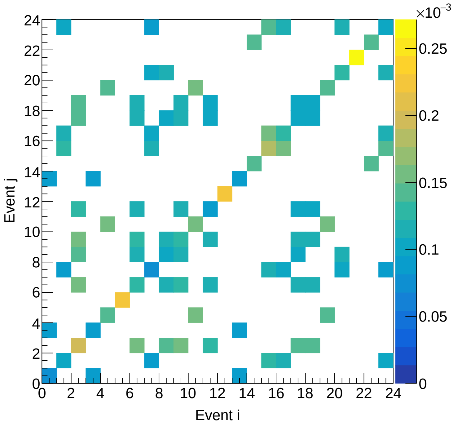
LD2 (total) Covariance | M: [5.7, 6.0) xF: [-0.05, 0.00)
